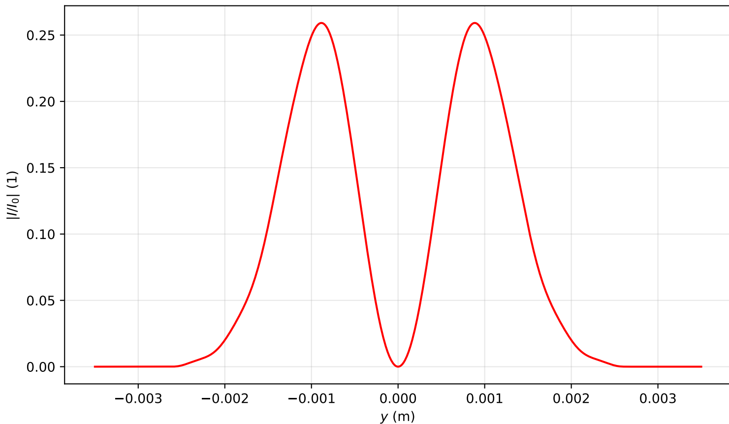
Intensity profile I(x=0, y, z=3.184)/I_0 , P_{in}=1.0P_{cr} , artificial time
